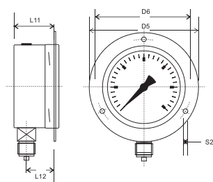
GAUGES WITH BOTTOM CONNECTION
