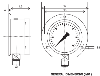
GENERAL DIMENSIONS (MM)
