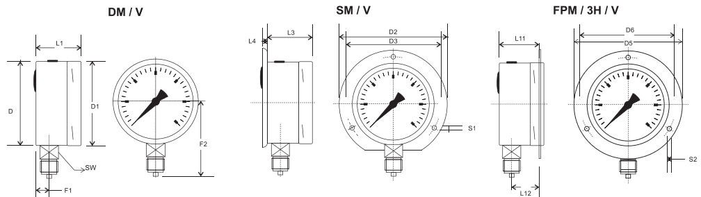
GAUGES WITH BOTTOM CONNECTION
